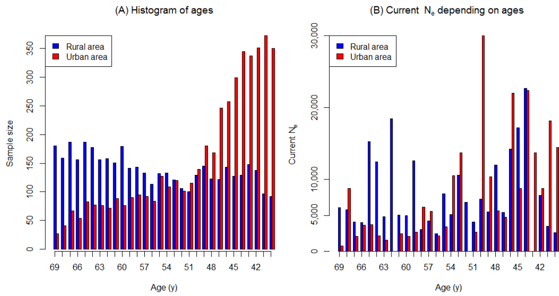
Supplementary Fig 3. (A) Histogram of ages depending on region. (B) Current N_e estimates depending on age and region (negative estimates were excluded in the plot).
