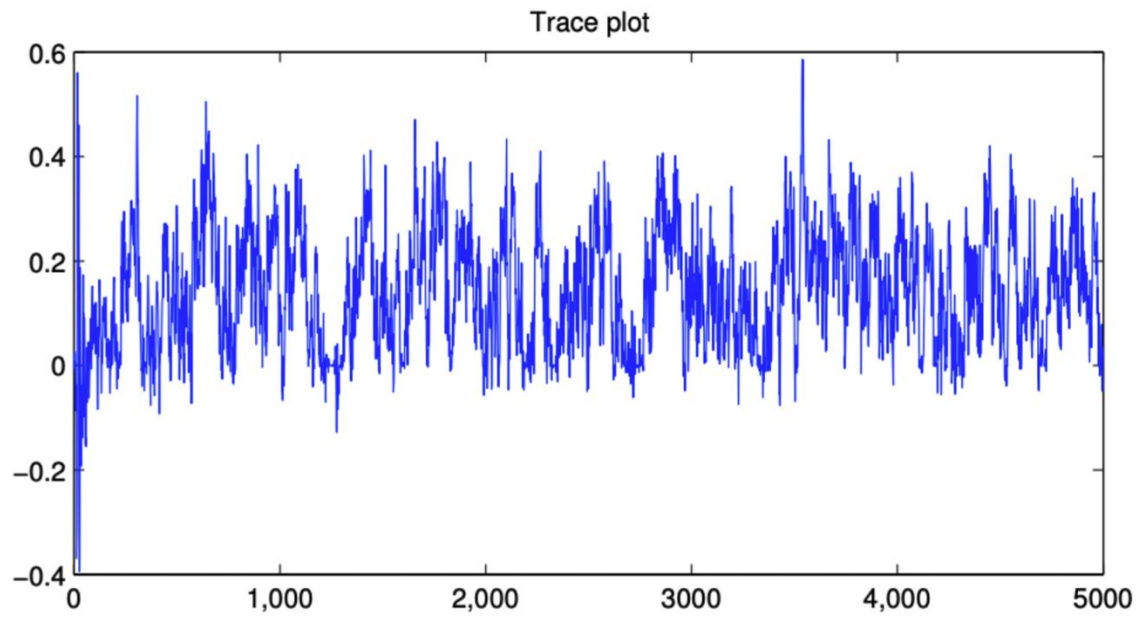
Supplementary Fig. 3. Trace plot of the regression coefficients \theta_{1,3} of the first selected SNP-set for 5,000 iterations of the MCMC algorithm. SNP, single nucleotide polymorphism; MCM, Markov chain Monte Carlo.
