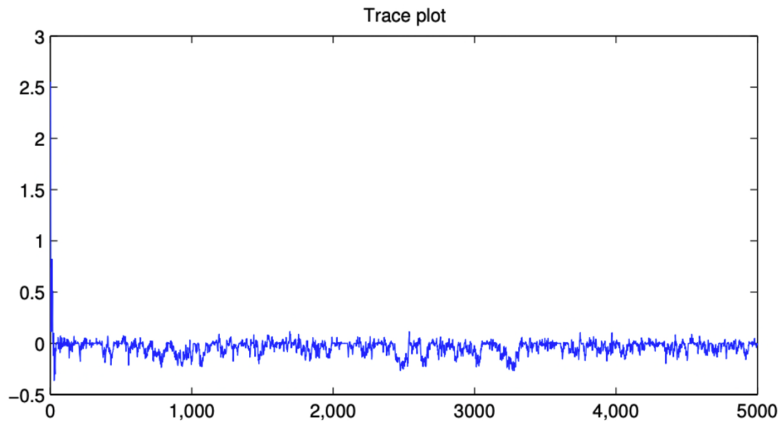
Supplementary Fig. 2. Trace plot of the regression coefficients \theta_{1,2} of the first selected SNP-set for 5,000 iterations of the MCMC algorithm. SNP, single nucleotide polymorphism; MCM, Markov chain Monte Carlo.
