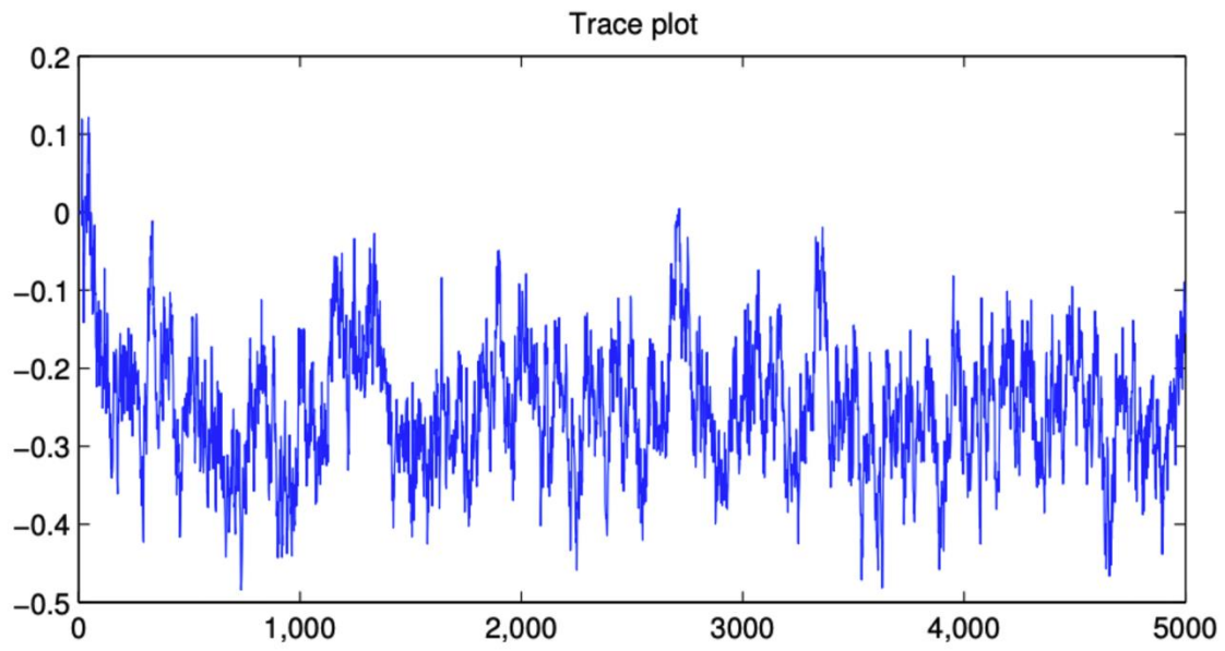
Supplementary Fig. 1. Trace plot of the regression coefficients \theta_{1,1} of the first selected SNP-set for 5,000 iterations of the MCMC algorithm. SNP, single nucleotide polymorphism; MCM, Markov chain Monte Carlo.
