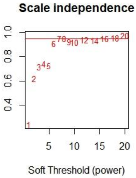
Supplementary Fig. 1. Scale independence and mean connectivity of R^2 and various soft thresholds.
