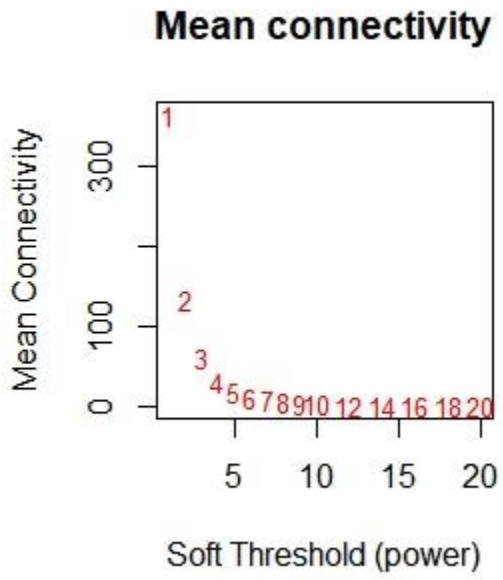
Supplementary Fig. 1. Scale independence and mean connectivity of R^2 and various soft thresholds.
