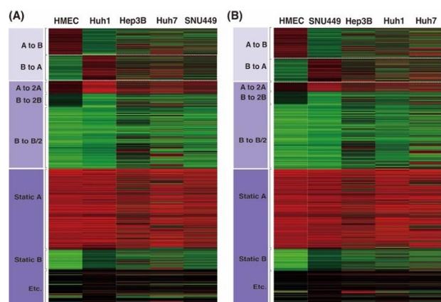
Supplementary Fig. 2. Distinguishing compartment landscapes in hepatocellular carcinoma cell lines. Heatmaps of compartment scores in each cell type, sorted according to compartment alteration. (A) The genomic bins were sorted by compartmental changes between human mammary epithelial cells (HMECs) and Huh1 cells. (B) The genomic bins were sorted by compartmental changes between HMECs and SNU449 cells.
