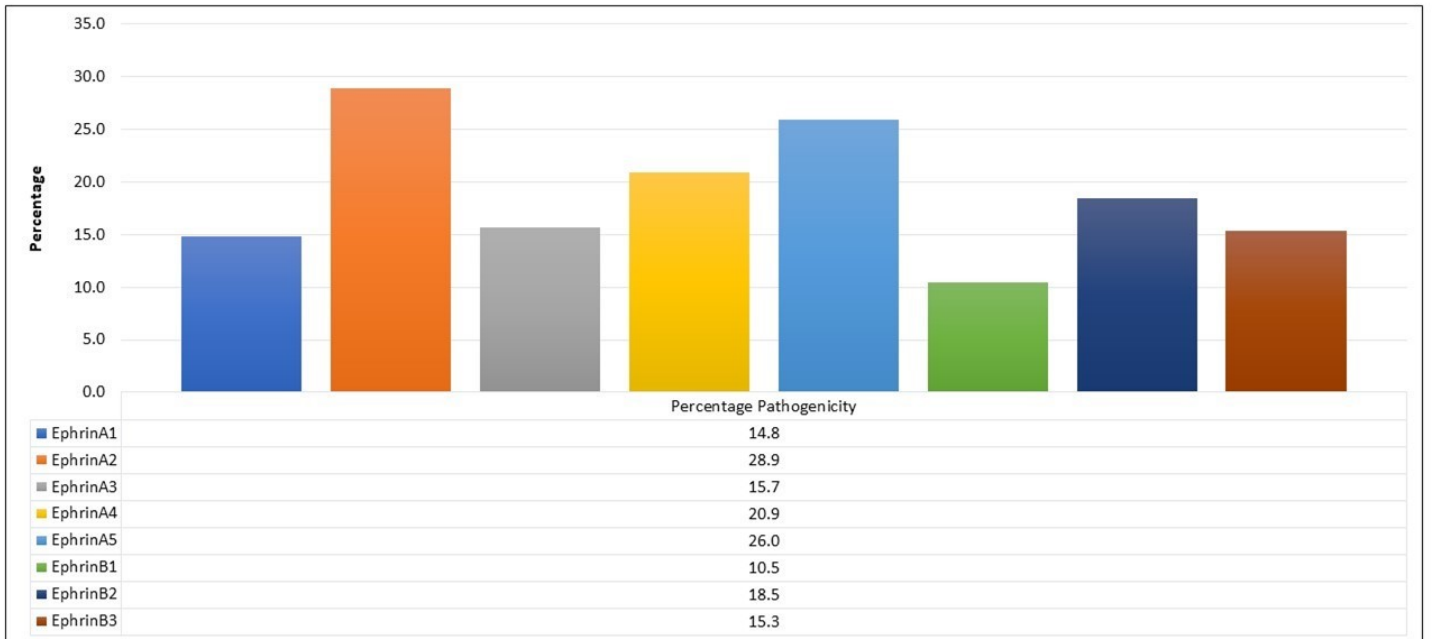
Supplementary figure 1 – Percentage of pathogenic mutations in (a) Ephrin A and (b) Ephrin B
