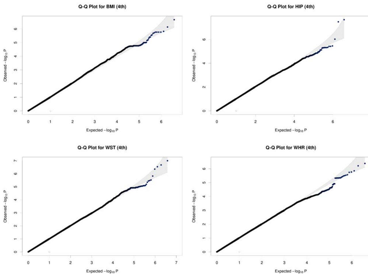
Supplementary Fig. 9. Quantile-Quantile plots of -\log_{10}(\text{p-value}) for association with cross-sectional fourth body mass index (BMI), hip circumference (HIP), waist circumference (WST), and waist-hip ratio (WHR) measurements using BOLT-LMM.
