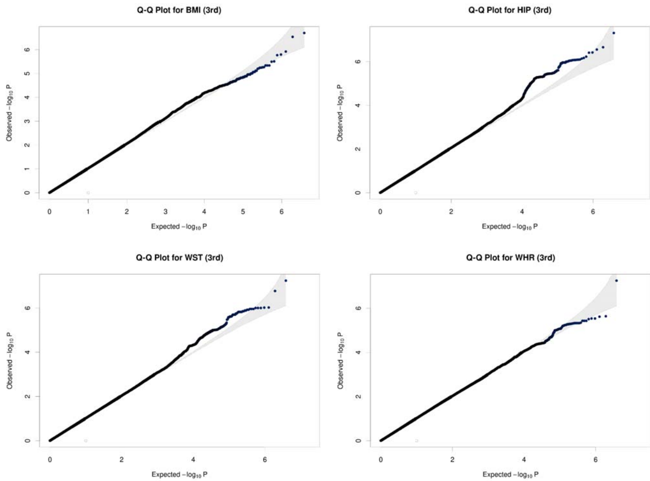
Supplementary Fig. 8. Quantile-Quantile plots of -\log_{10}(\text{p-value}) for association with cross-sectional third body mass index (BMI), hip circumference (HIP), waist circumference (WST), and waist-hip ratio (WHR) measurements using BOLT-LMM.
