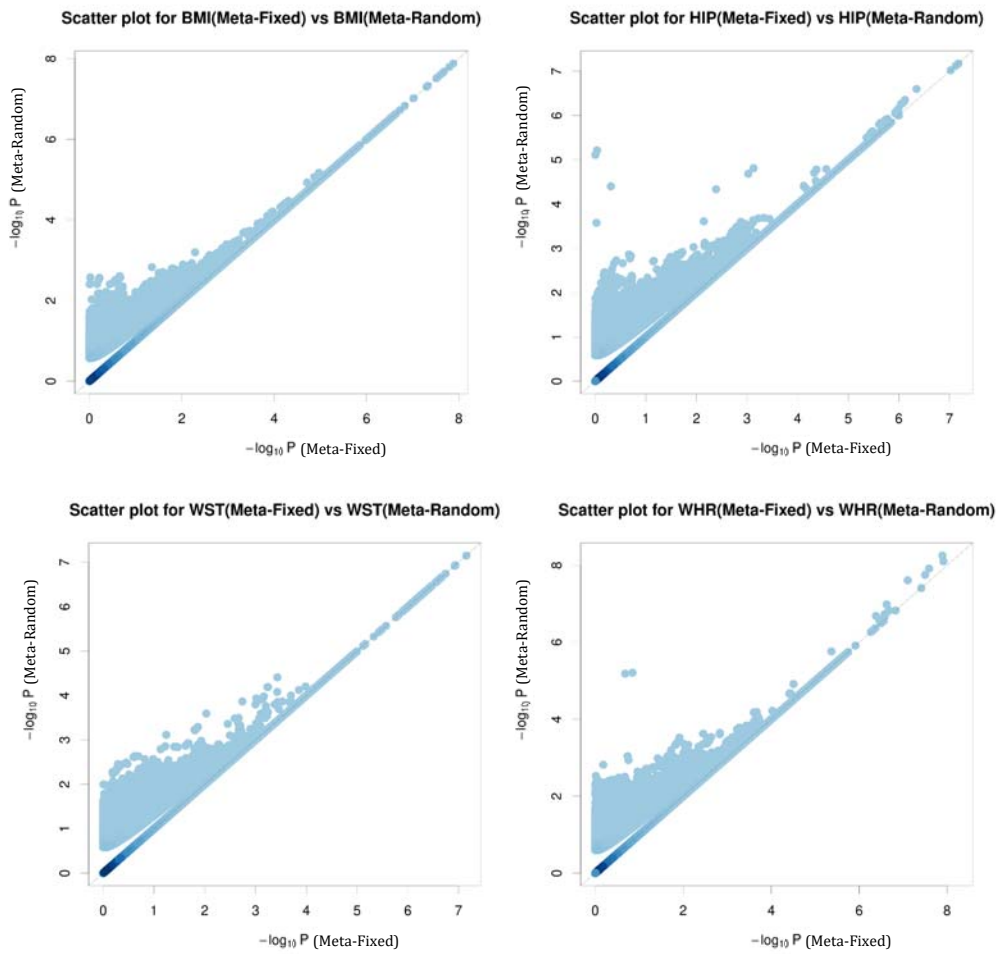
Supplementary Fig. 19. Scatter plots of -\log_{10}(\text{P-value}) for association for longitudinal body mass index (BMI), hip circumference (HIP), waist circumference (WST), and waist-hip ratio (WHR) measurements between Meta-Random method vs. Meta-Fixed Method.
