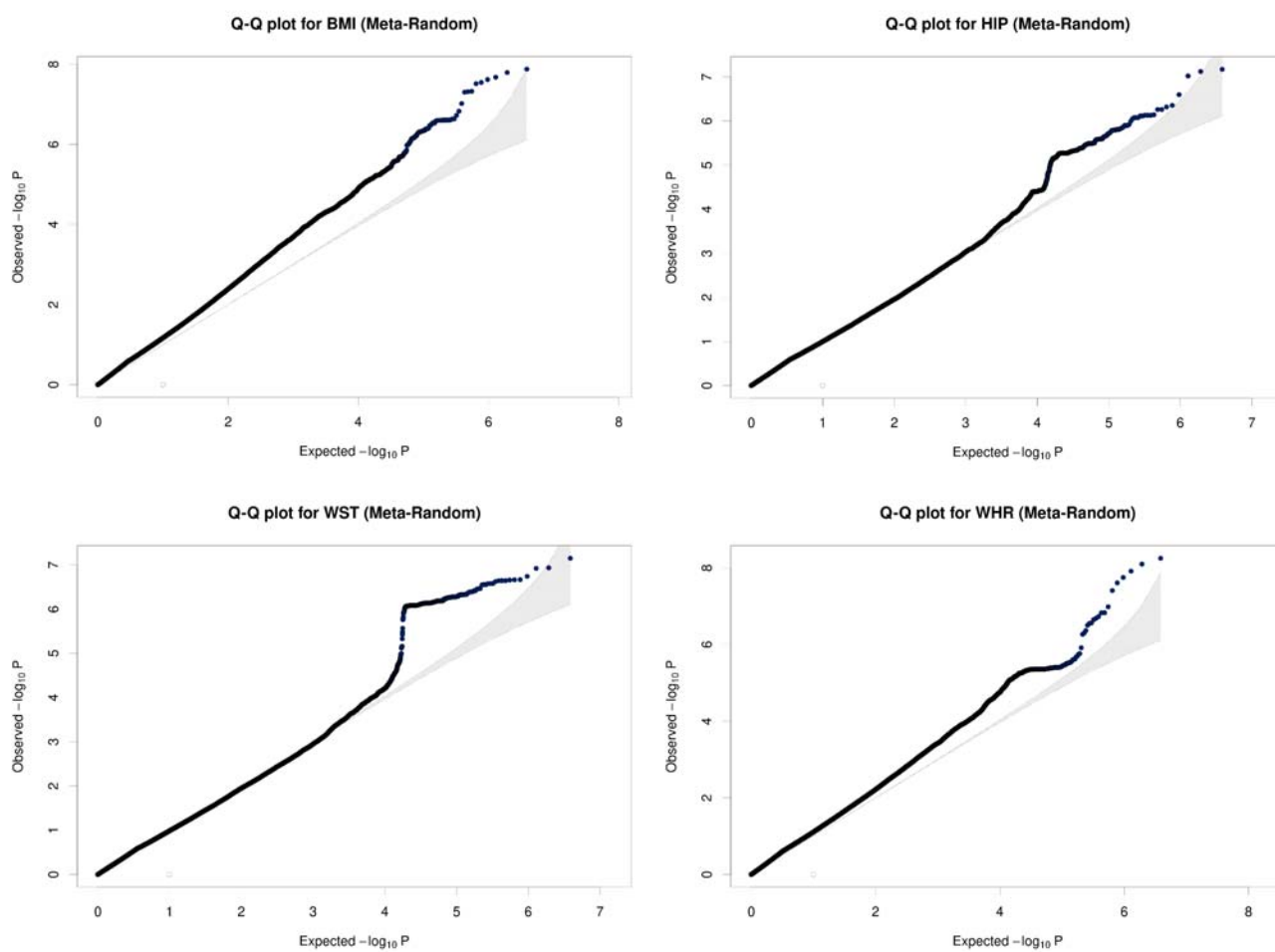
Supplementary Fig. 18. Quantile-Quantile plots of -\log_{10}(\text{p-value}) for association with longitudinal body mass index (BMI), hip circumference (HIP), waist circumference (WST), and waist-hip ratio (WHR) measurements using Meta-Random method.
