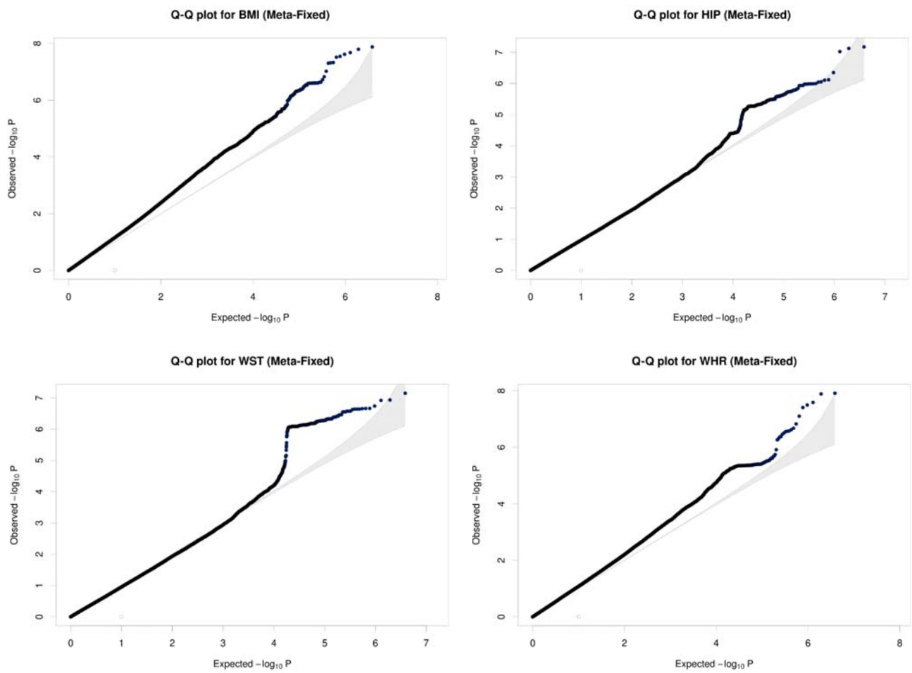
Supplementary Fig. 17. Quantile-Quantile plots of -\log_{10}(\text{p-value}) for association with longitudinal body mass index (BMI), hip circumference (HIP), waist circumference (WST), and waist-hip ratio (WHR) measurements using Meta-Fixed method.
