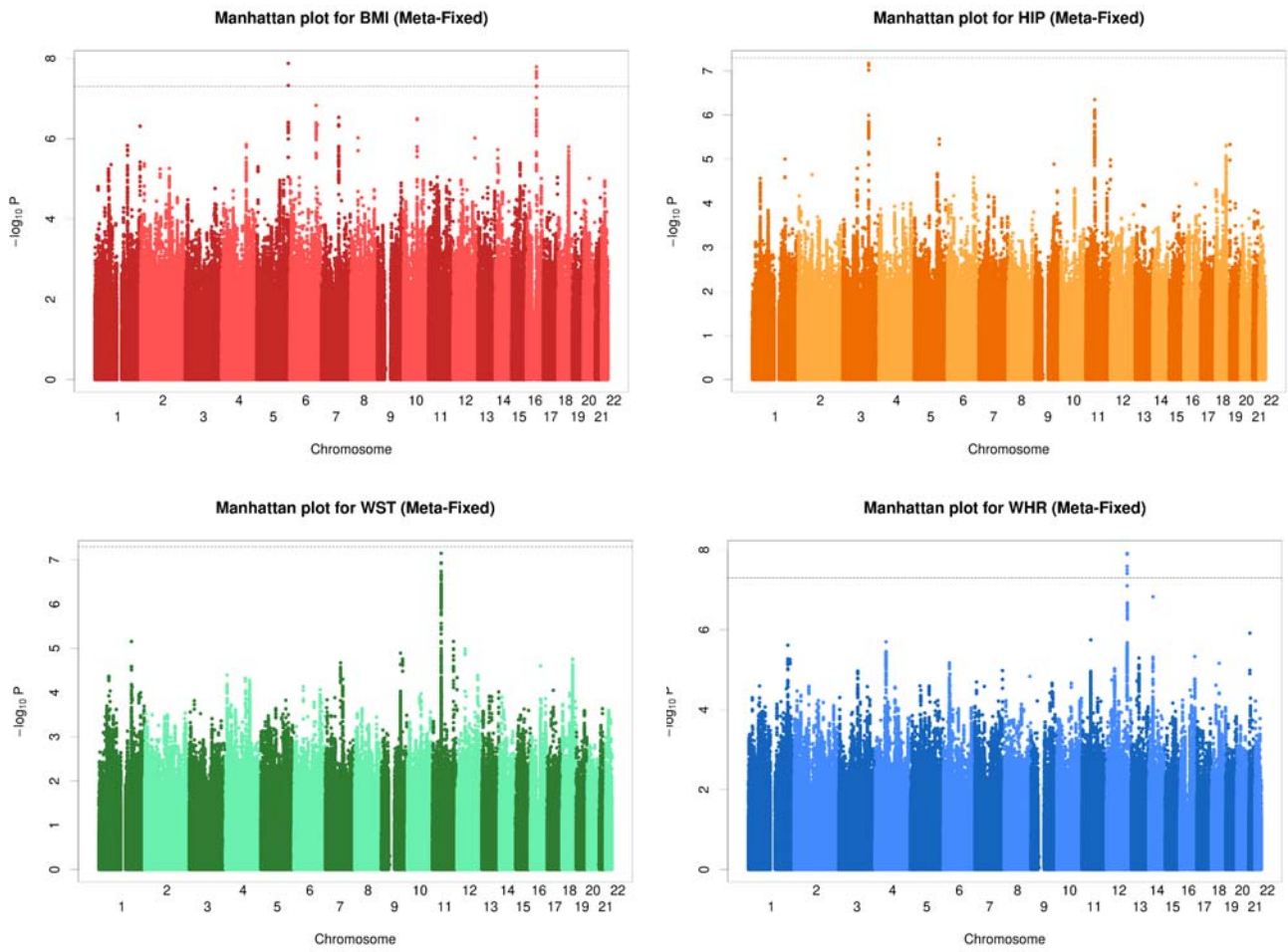
Supplementary Fig. 16. Genomewide Manhattan plots of -\log_{10}(\text{p-value}) for association with longitudinal body mass index (BMI), hip circumference (HIP), waist circumference (WST), and waist-hip ratio (WHR) measurements using Meta-Fixed method.
