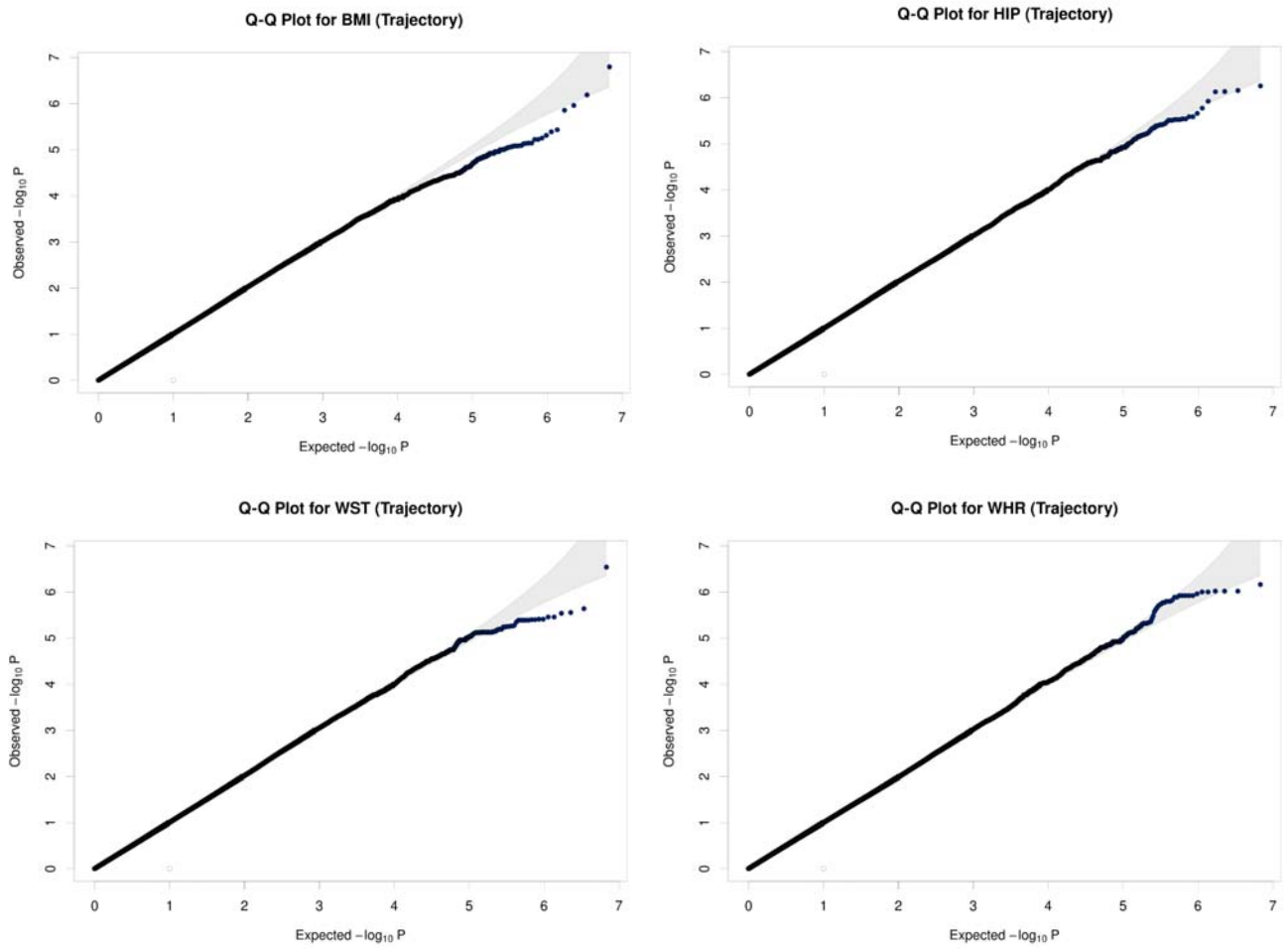
Supplementary Fig. 15. Quantile-Quantile plots of -\log_{10}(\text{p-value}) for association with trajectory body mass index (BMI), hip circumference (HIP), waist circumference (WST), and waist-hip ratio (WHR) measurements using BOLT-LMM.
