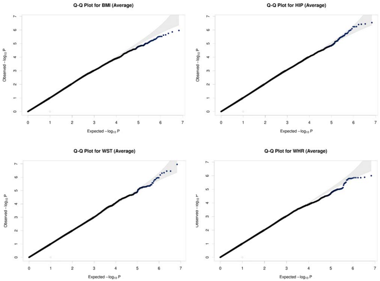
Supplementary Fig. 14. Quantile-Quantile plots of -\log_{10}(p\text{-value}) for association with average body mass index (BMI), hip circumference (HIP), waist circumference (WST), and waist-hip ratio (WHR) measurements using BOLT-LMM.
