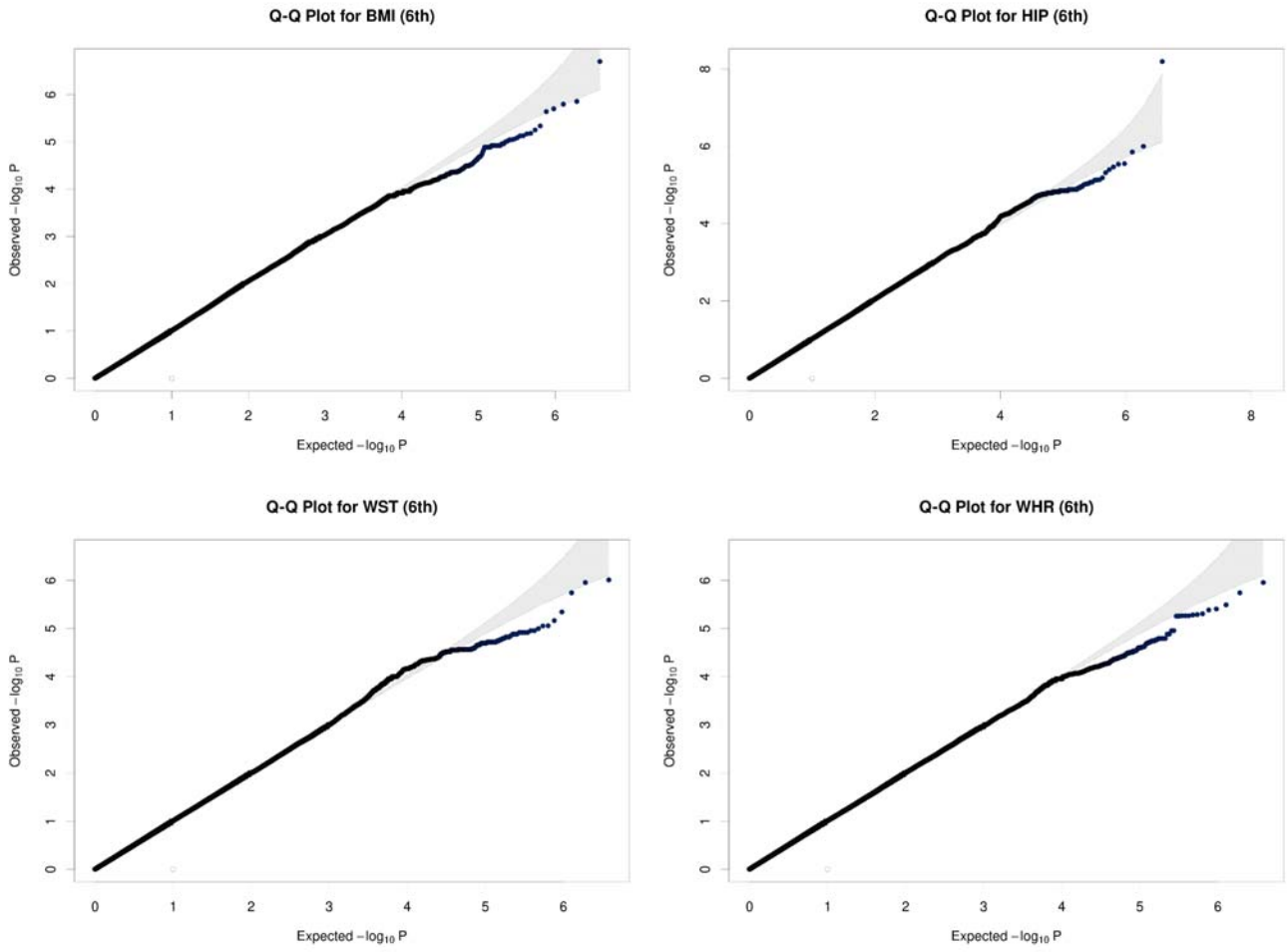
Supplementary Fig. 11. Quantile-Quantile plots of -\log_{10}(\text{p-value}) for association with cross-sectional sixth body mass index (BMI), hip circumference (HIP), waist circumference (WST), and waist-hip ratio (WHR) measurements using BOLT-LMM.
