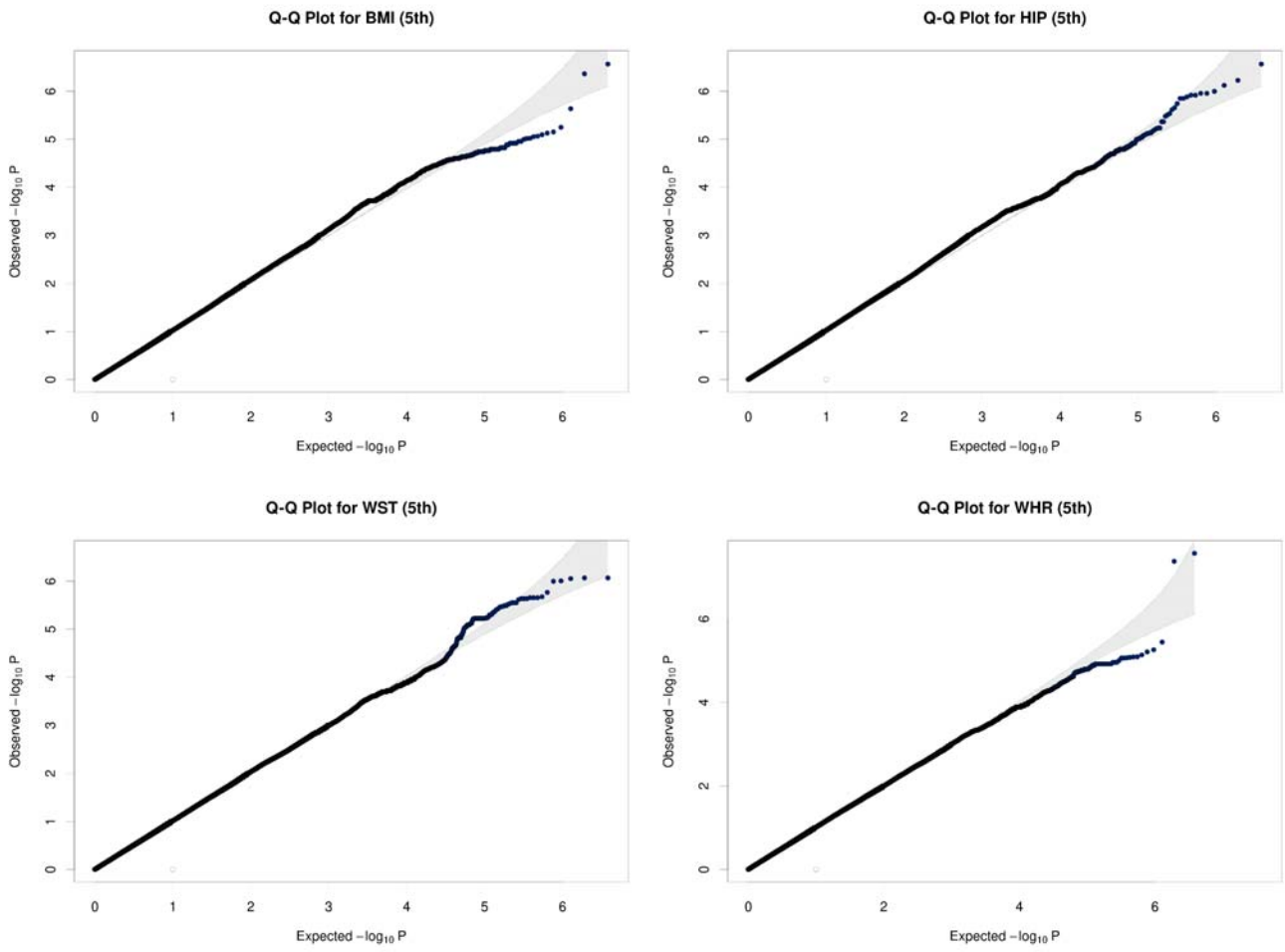
Supplementary Fig. 10. Quantile-Quantile plots of -\log_{10}(\text{p-value}) for association with cross-sectional fifth body mass index (BMI), hip circumference (HIP), waist circumference (WST), and waist-hip ratio (WHR) measurements using BOLT-LMM.
