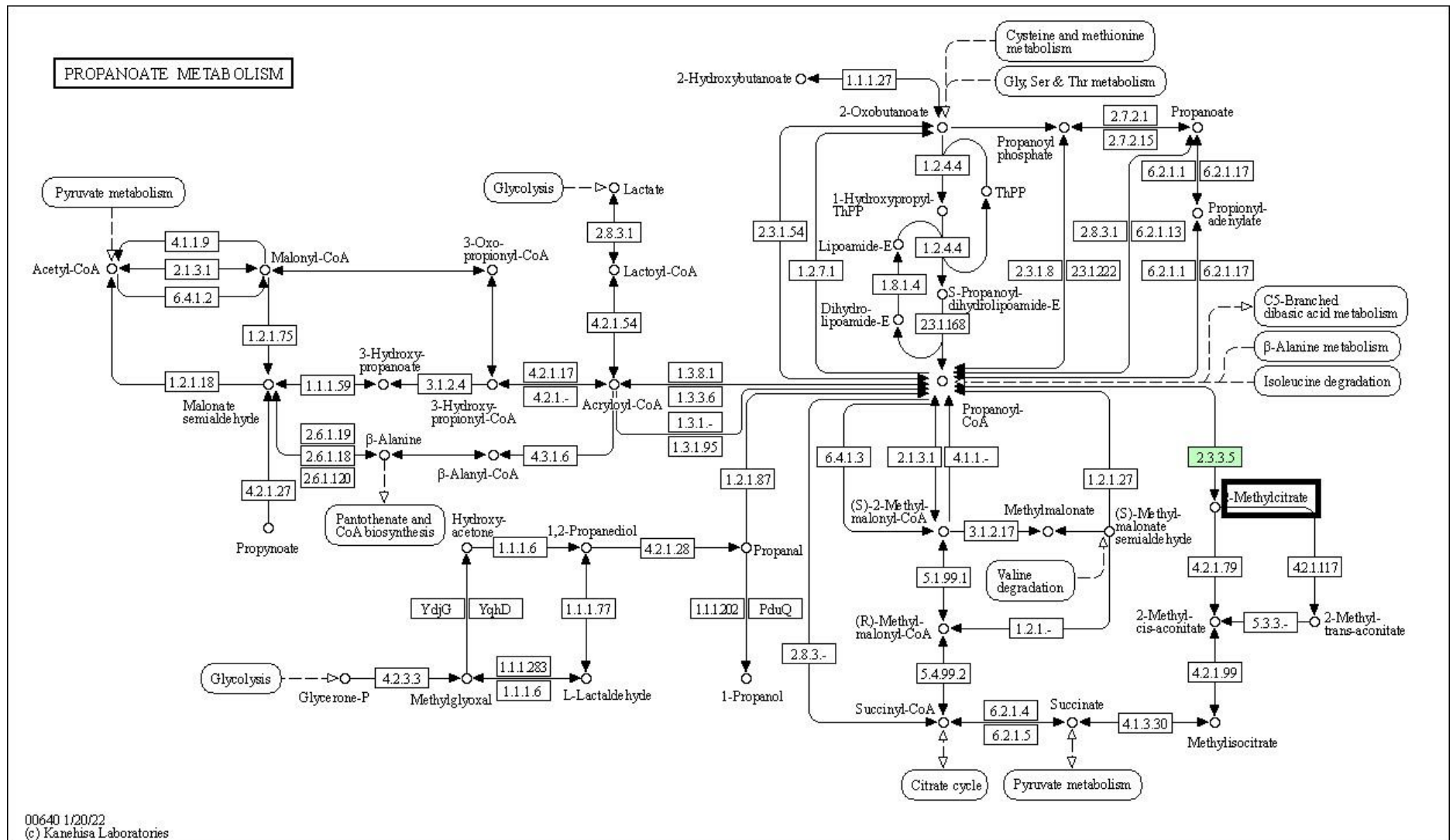
Supplementary Fig. 2. Potential metabolic pathways associated with the virulence protein WP_013745346.1 by KAAS (KEGG automatic annotation server analysis).
