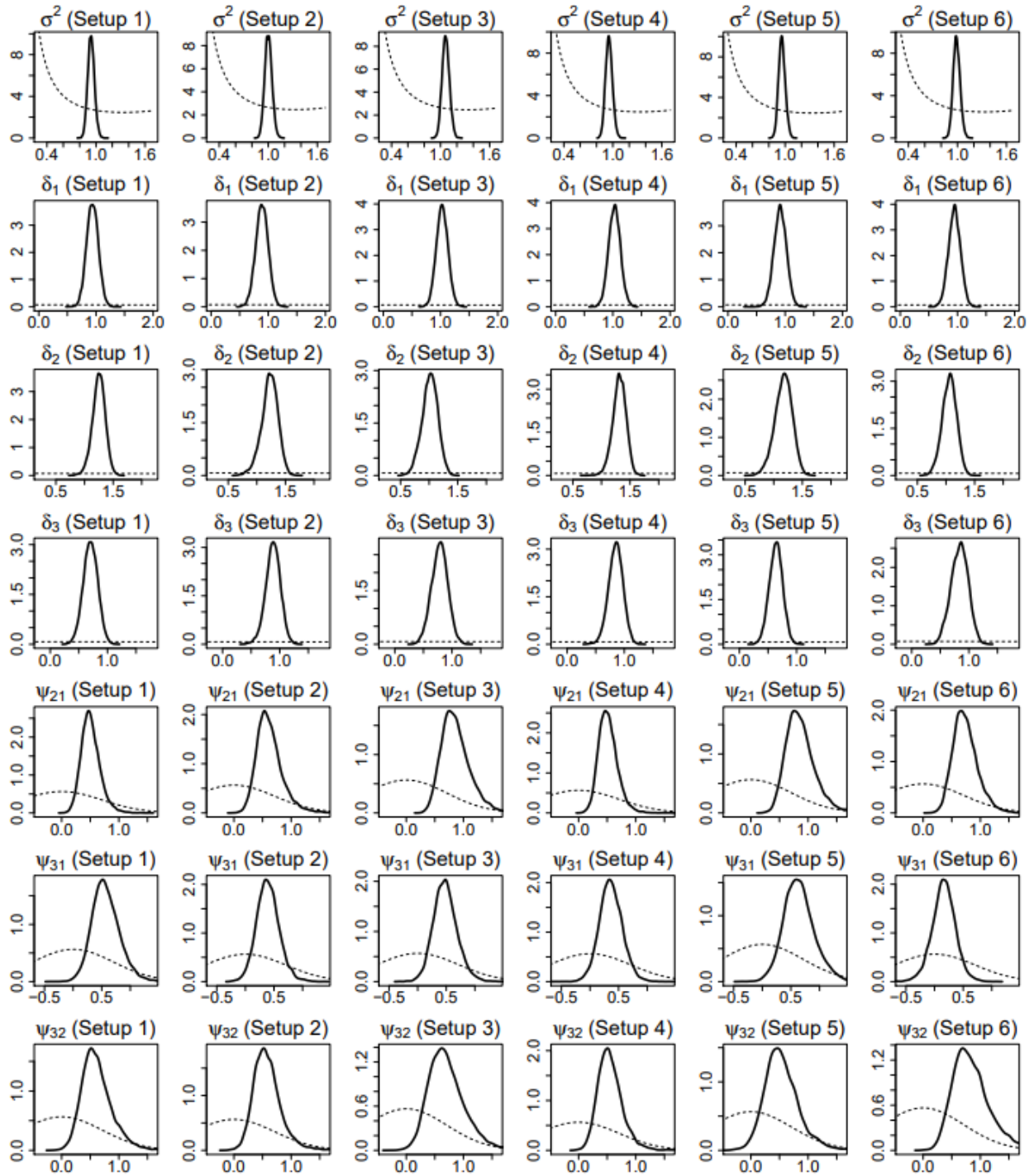
Supplementary Fig. 3. Posterior (solid line) and prior (dashed line) densities of the parameters for random errors and random effects for Setups 1–6. Estimated densities are based on 10,000 random draws.
