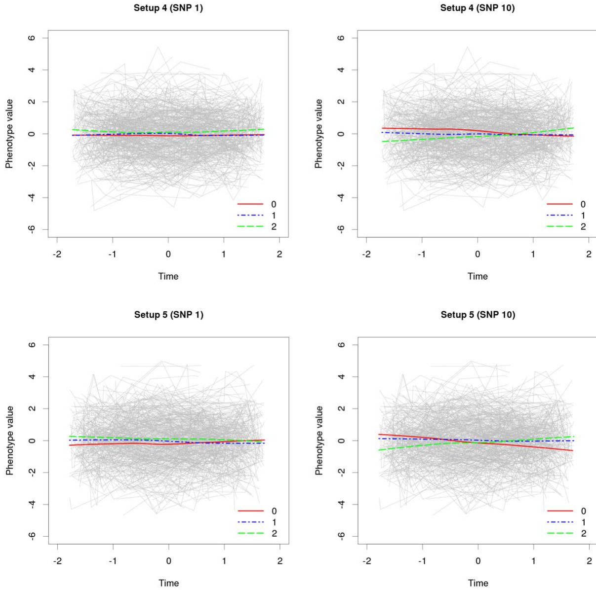
Supplementary Fig. 1. Time-dependent curves of averaged phenotype values for three different genotypes (0, 1, 2) at 1st causal single nucleotide polymorphism (SNP) with no SNP-time interaction and 10th causal SNP with SNP-time interaction for Setups 4 and 5.
