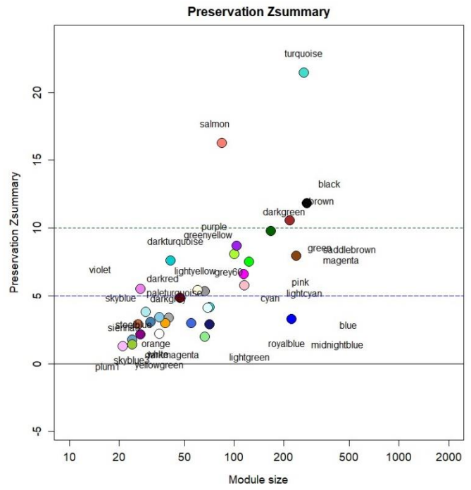
Supplementary Fig. 2. Z_{\text{summary}} score.
